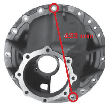
MAIN HOUSING
