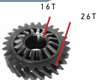
BULL GEAR 3RD DIFF 60mm & 64mm
