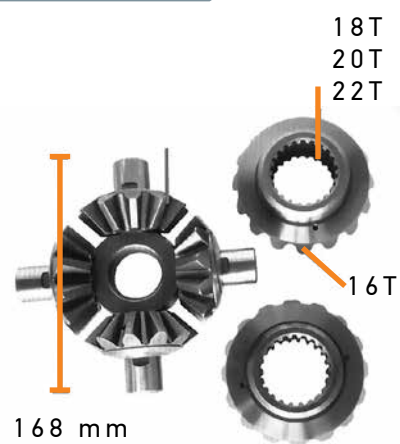
SIDE GEAR SPIDER GEAR CROSS SHAFT
