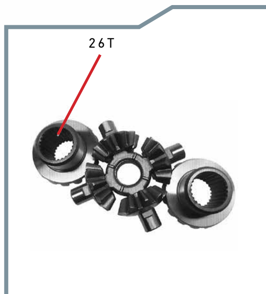
SIDE GEAR SPIDER GEAR CROSS SHAFT
