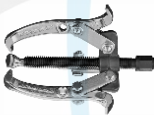
11-859 Gear Puller 3 Jaw 300mm
