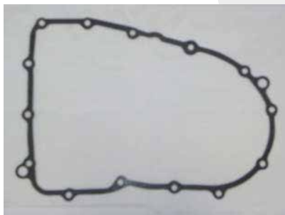
48704 K48900X CASE ID: HM-3 SPEED 190-82 ACCORD, PRELUDE OEM #21811-PA9-000/010
