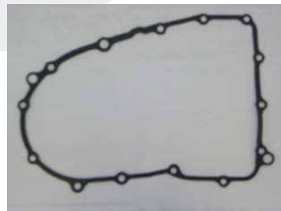
48704A K48900X CASE ID: HM-3 SPEED 190-82 ACCORD, PRELUDE, 1981-83 CIVIC OEM #21811-PA9-020
