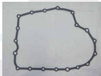
98424 K98900D CASE ID: SPCA, MPKA 2006-12 CIVIC OEM #21811-RPC-000
