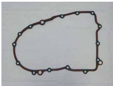
48706B K48900A, K48900X CASE ID: AK, A5 1983-87 PRELUDE, 1983-85 ACCORD, 1984-85 CIVIC, CRX (3 SP) OEM #21811-PLY-000/S00
