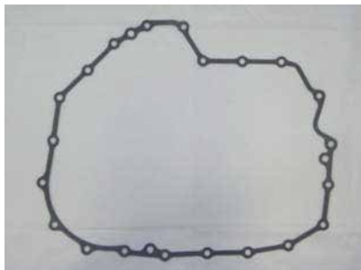
98151 K98900L CASE ID: SLSA, S5RA, SWRA, SG0A 2001-12 NON-USA CVT FIT, JAZZ, CITY & AIRWAVE OEM #21811-PWR-000
