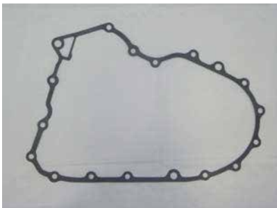
48827 K48900J, 48900C CASE ID: MP7A, SP7A, BDRA, S4RA, A4RA, B46A, S4XA, M4RA, B4RA, SKWA, A24A, M24A, S24A 1994-01 INTEGRA, 1992-00 CIVIC OEM 321811-P56-000, 21811-P24-000
